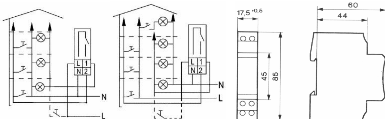
Wiring diagram
